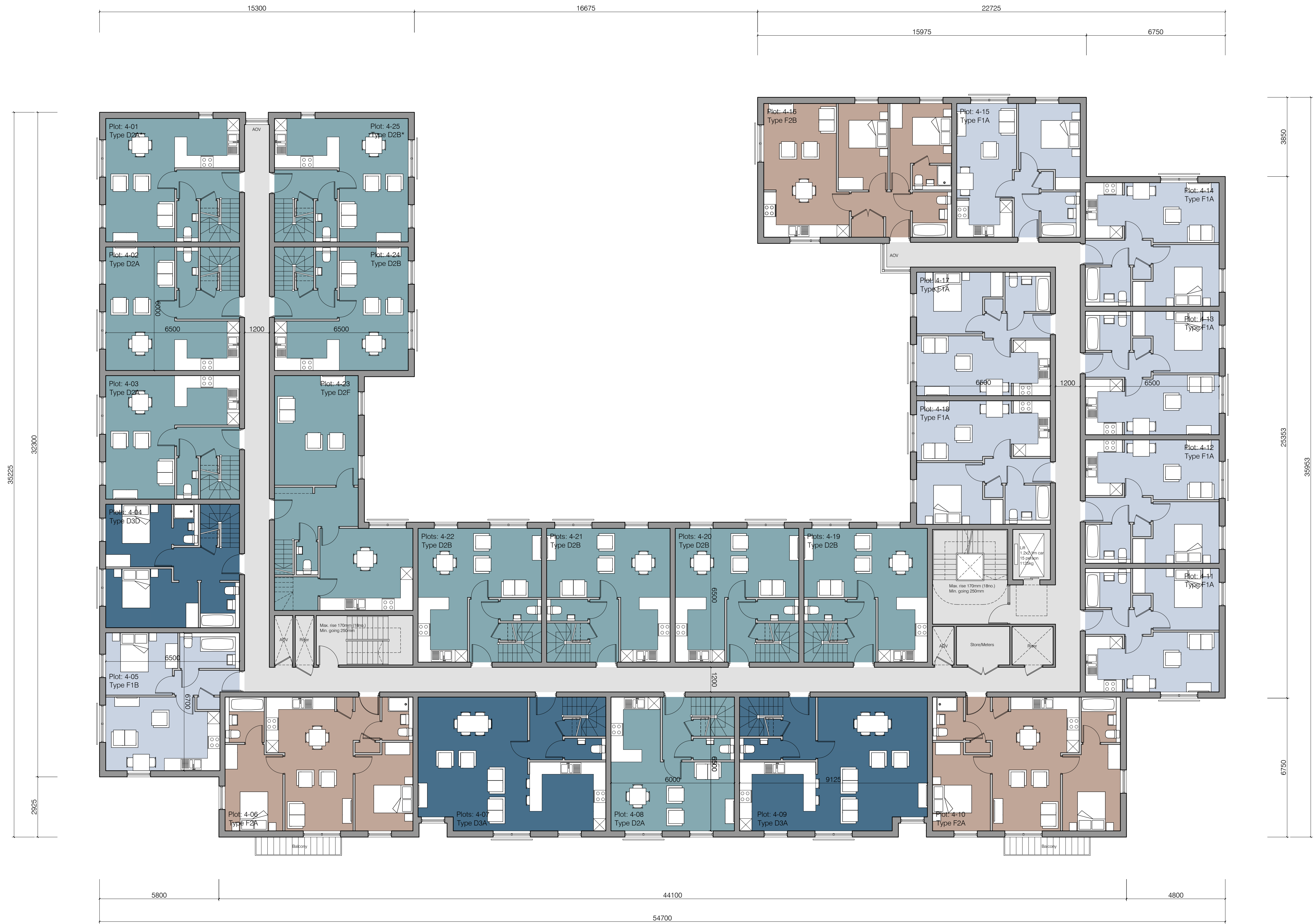
Fourth Floor Block Layout +13.2m
