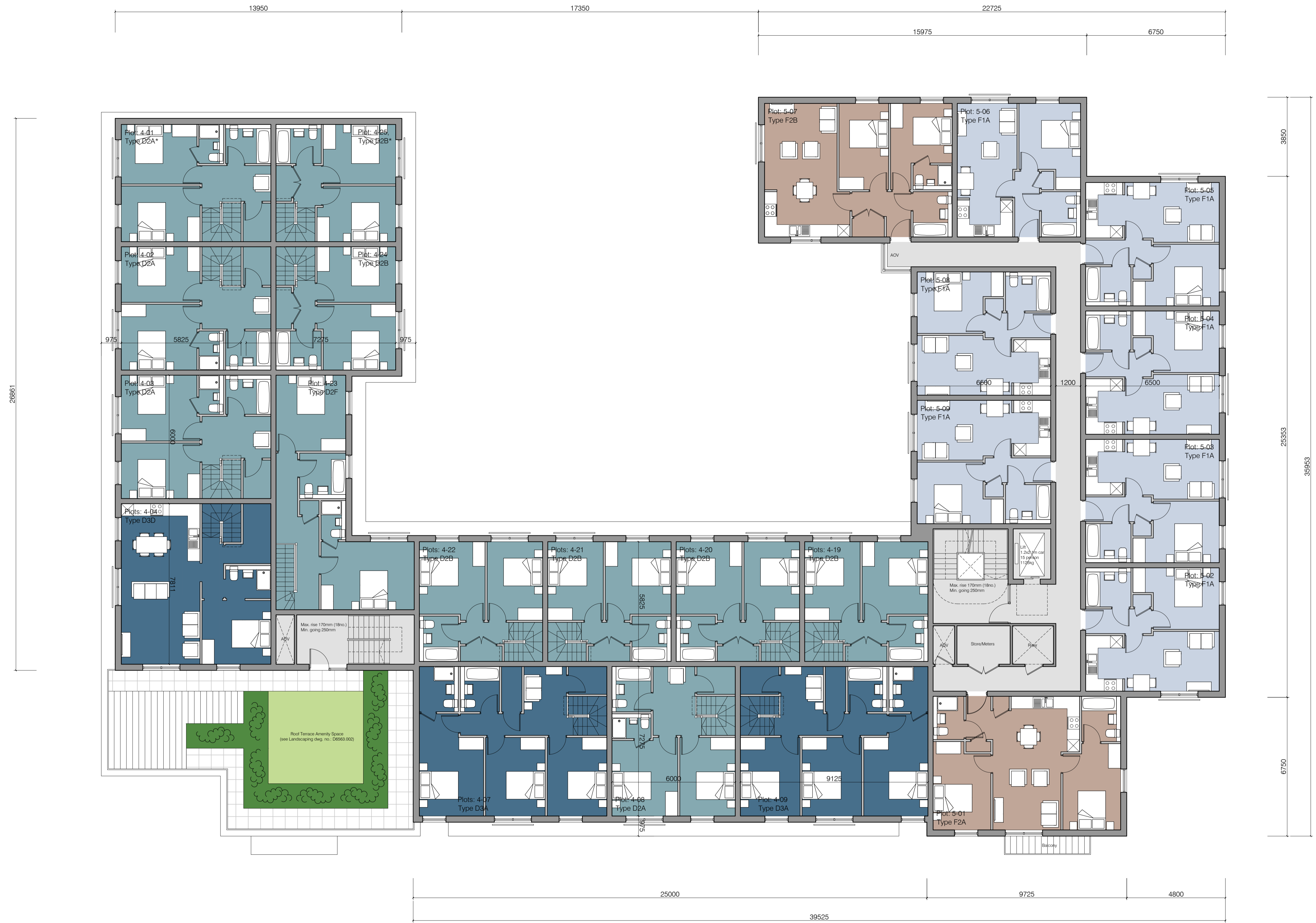
Fifth Floor Block Layout +16.2m
